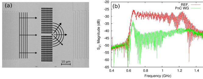
Figure 1. (a) Scanning electron microscope image of a phononic waveguide device with an eight-period long crystal consisting of a square lattice of air holes etched into lithium niobate. The chirped transducers are visible at the left and right edges of the picture. A schematic drawing of the expected wavefronts launched by the source transducer and as leaving the structure after propagation through the waveguide are also shown. (b) Transmission response of the phononic waveguide structure, expressed in terms of S_{21} scattering parameters, together with the response of a similar structure without a phononic crystal (an electro-acoustic delay line) used as a reference. Note that the receiving transducer is designed to sense SAWs with straight phase fronts and is thus insensitive to the cylindrical SAWs exiting from the waveguide.
