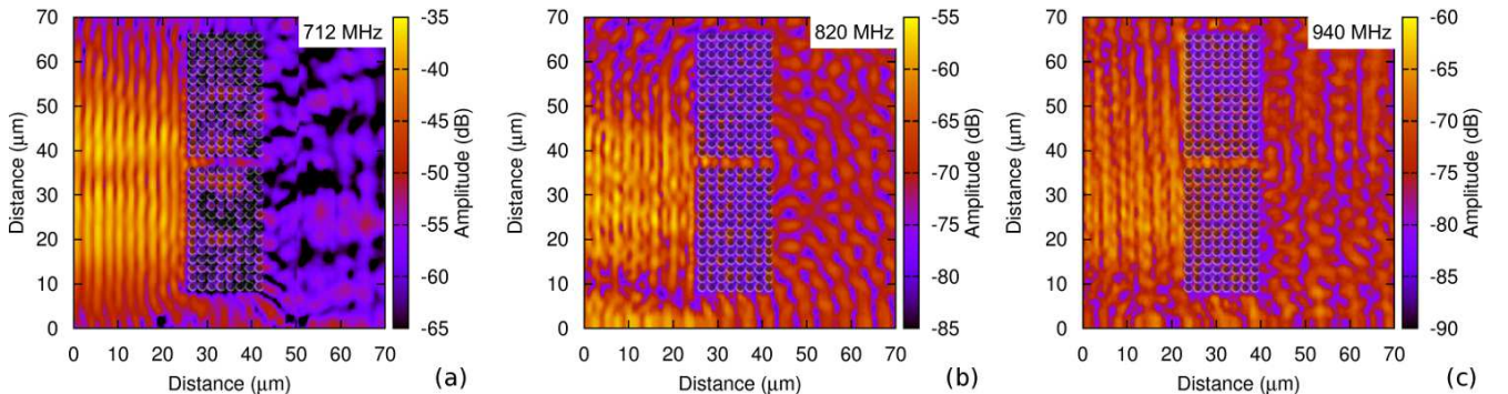
Figure 2. Measured elastic wave field amplitude maps for excitation frequencies located (a, b) inside (712 and 820 MHz) and (c) at the output (940 MHz) of the band gap. The scans cover an area of 70 \mu\text{m} \times 70 \mu\text{m} with an 0.5 \mu\text{m} step size. A semi-transparent scanning electron microscope picture of the holes overlays the measurement data as a guide for the eye. Phonon wave guiding is observed in (b) and (c).
