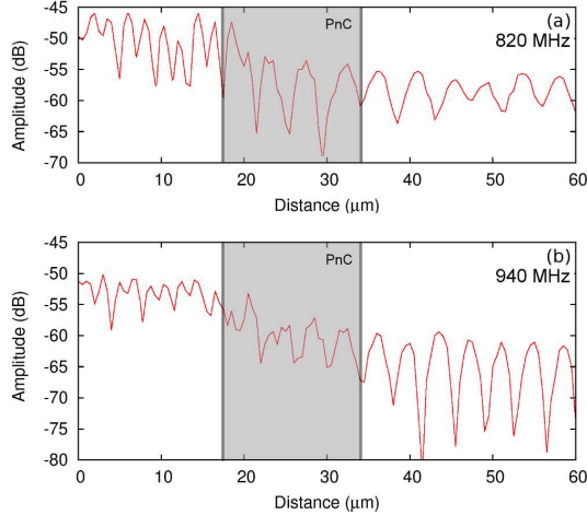
Figure 3. Amplitude line profiles measured inside the phononic waveguide and along the propagation direction taken at (a) 820 and (b) 940 MHz. The shaded area indicate the position of the phononic crystal (PnC).
