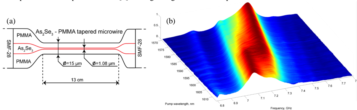
Fig. 1 (a) Scheme of the hybrid \text{As}_2\text{Se}_3 -PMMA optical microwire used to observe avoided crossing effects. (b) Experimental Brillouin backscattering spectrum as a function of pump wavelength showing the nonlinear frequency gap due to avoided crossing at a pump wavelength of 1600 nm.
