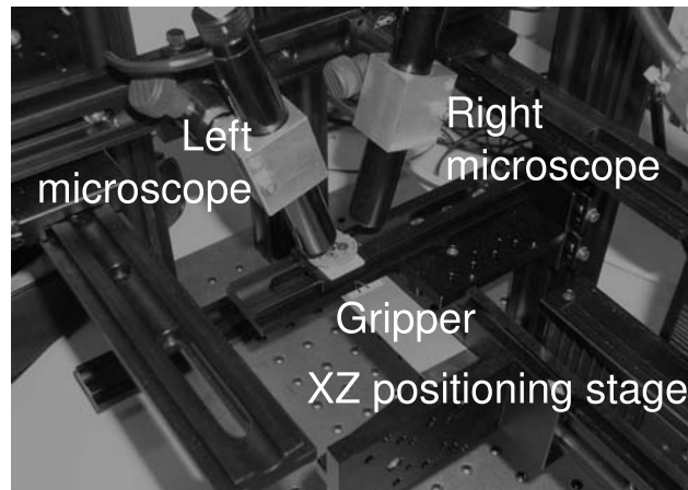
Figure 2: Experimental setup.
