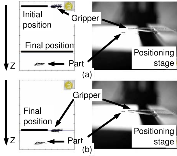
Figure 13: Positioning of the gripper with respect to the part: (a) virtual and real initial views, respectively (b) virtual and real final views, respectively.
