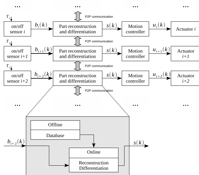
Fig. 2. The distributed control architecture.
