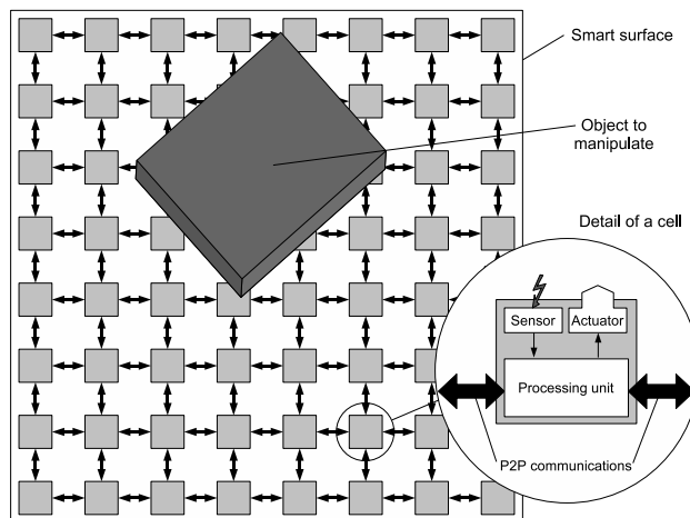
Fig. 1. The Smart Surface concept.
