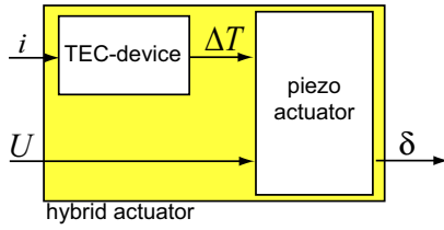
Fig. 4. Systemic scheme of the hybrid microactuator.
