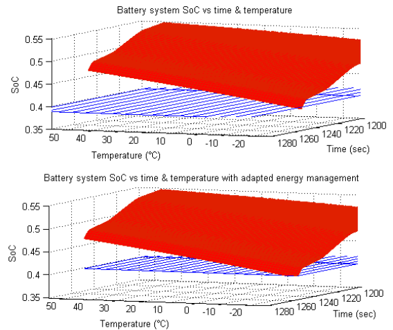
Fig. 15. Evolution of battery system SoC vs.time and temperature, without and with adapted energy management
