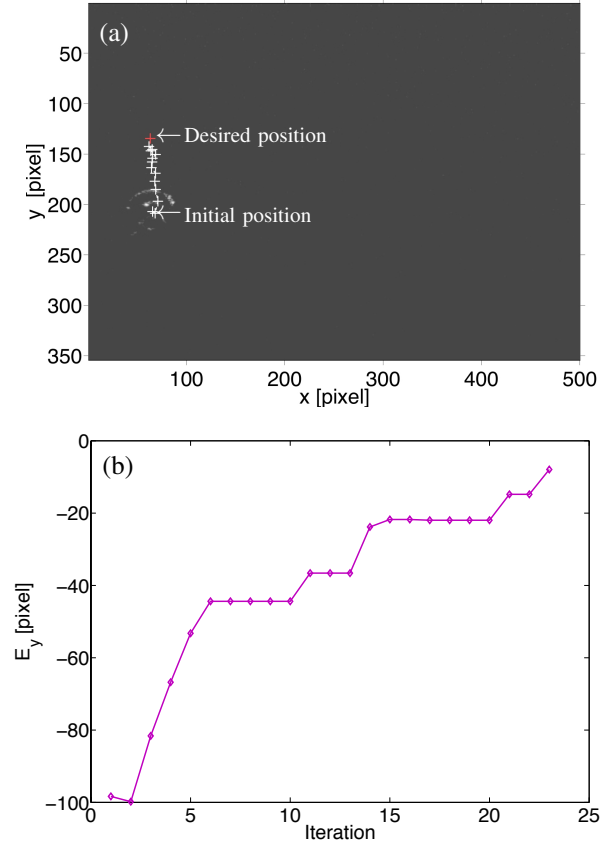
Fig. 9. 1D positioning: (a) along Y \lambda=0.2 , \xi=100 \mu\text{m} and (b) the evolution of the error e for 23 iterations.
