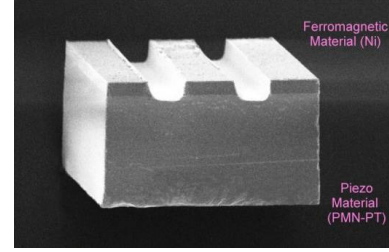
Fig.4 SEM of a MagPier microrobot type I.2 (trenches are 50 \mu\text{m} wide).
