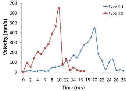
Fig. 12 Velocity characterizations of MagPieR type II.1 and II.2
