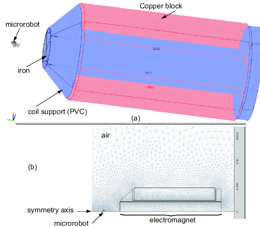
Fig.8: Comsol Multiphysics - FEM analysis. (a): scheme showing the geometrical characteristics and distance between the microrobot and the electromagnet. (b): 2D-axisymmetrical meshing.
