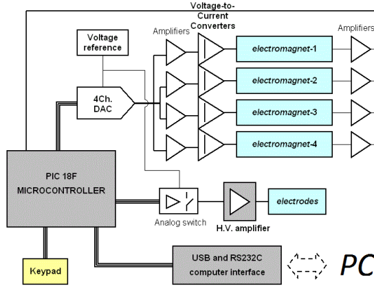
Fig.3 Block diagram of embedded electronic circuit
