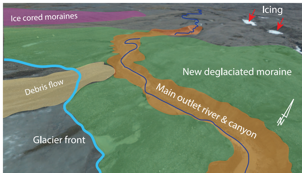
Figure 4. The newly deglaciated moraine consists in a 200 m wide strip at the front of the glacier (light green). It represents the glacial retreat over the last 10 years, and is the area where geomorphological processes are the most active. The location from which the picture was taken is indicated in Fig. 2 with the star named 4, with a viewing direction towards the North-West, giving a hint of the scale of the features visible here.
