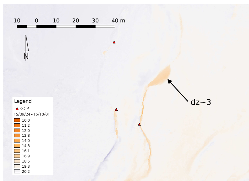
Figure 10. Difference of DEM (DoD) for assessing moraine movements due to a significant flood event, with one wall of the canyon collapsing between the two dates. The images for generating the DEMs were acquired September 24th 2015 and October 1st 2015. The landslide generated canyon collapse depth is about 3 m.
