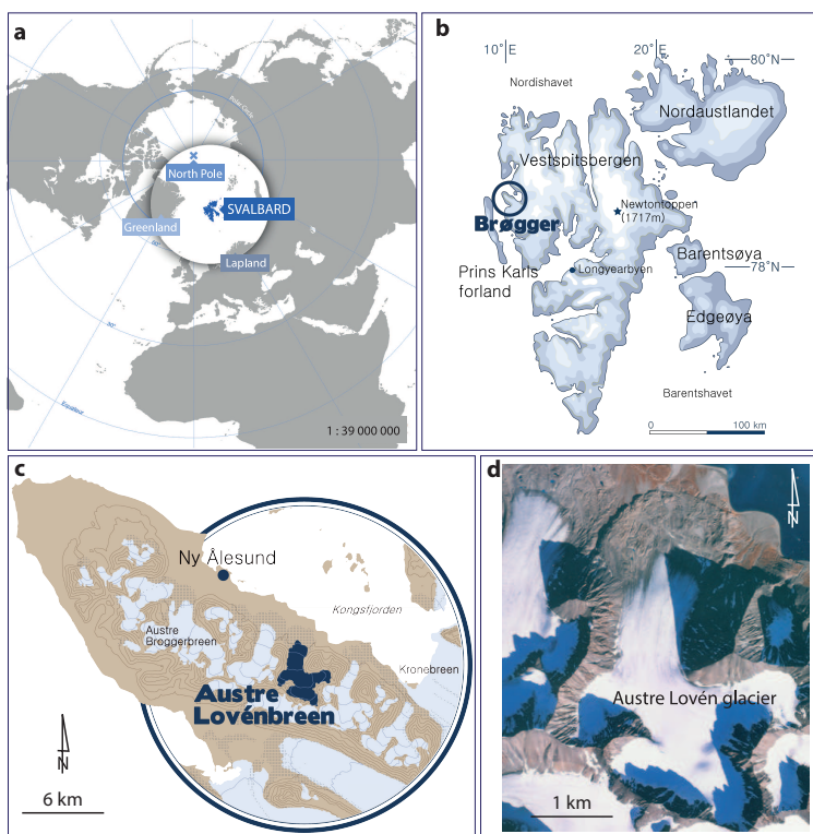
Figure 1. Field work is located in the high-Arctic, on the West coast of Spitsbergen. Austre Lovén is a small land terminating glacier, chosen by scientists since the early 60s for its geomorphological characteristics.
