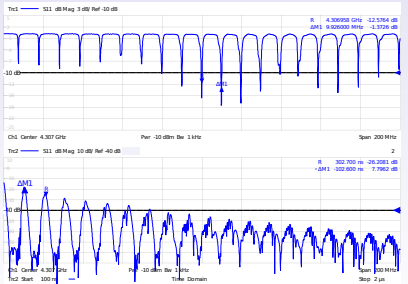
HBAR characterization
