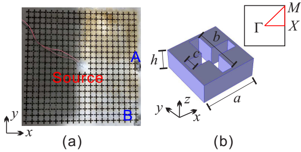
Figure 2: Phononic crystal slab sample manufactured in a stainless steel plate. (a) The Lamb wave source in the center is a piezoelectric patch. Transmitted waves are measured along the \Gamma X direction (at point A) and the \Gamma M direction (at point B). (b) The primitive unit cell is schematized, including geometrical dimensions and the first Brillouin zone for the square lattice.
