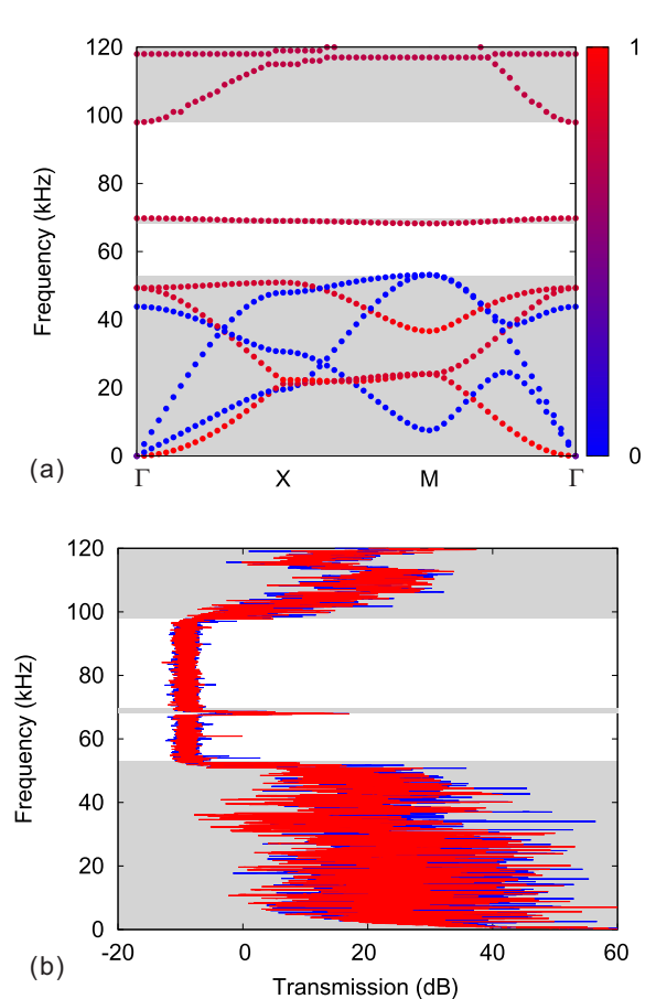
Figure 3: (a) Phononic band structure and (b) experimental transmission of the perfect PC slab with cross holes ( b/a = 0.9 , c/a = 0.2 , h/a = 0.4 ). The color scale in panel (a) measures the polarization and varies from in-plane modes (blue) to out-of-plane modes (red). The gray areas indicate the passing frequency ranges. The blue and red lines in panel (b) show measurements along the \Gamma X and \Gamma M directions, respectively.
