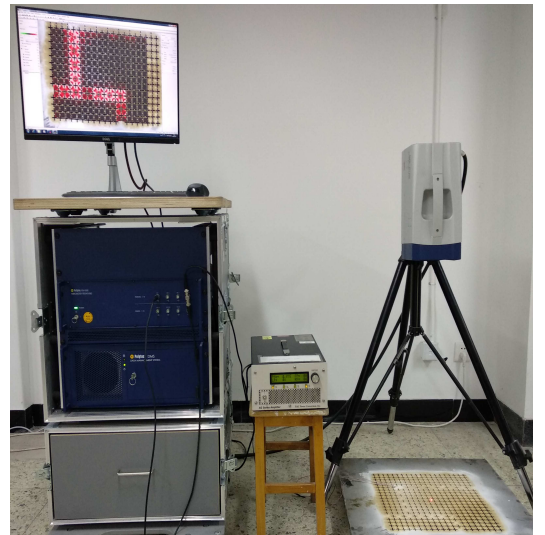
Figure 1: Photograph of the experimental setup illustrating the measurement of vertical displacements of Lamb waves excited in a phononic crystal slab sample.
