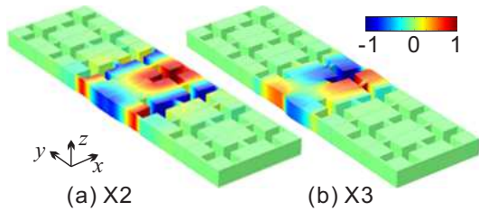
Figure 7: Distribution of the x -displacement at the X point for Bloch waves 2 and 3 in Fig. 6(a). The color scale varies from negative (blue) positive (red) normalized values.
