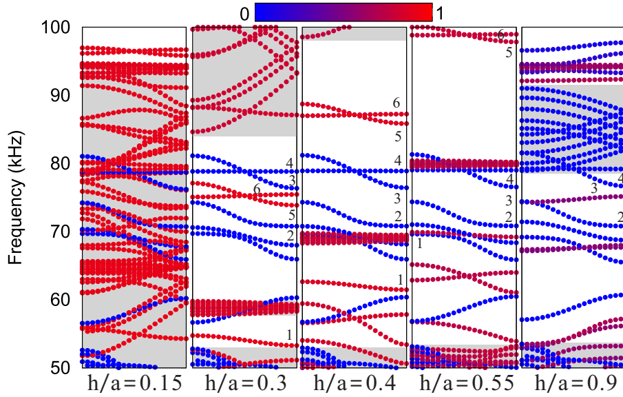
Figure 8: Band structures of CREWs with different relative thicknesses ( b/a = 0.9 , c/a = 0.2 ). The color scale measures the polarization and varies from in-plane modes (blue) to out-of-plane modes (red). The gray areas indicate the passing bands for the corresponding perfect PC slab.
