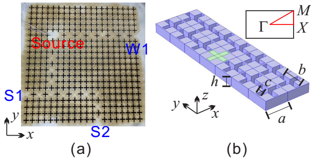
Figure 4: Coupled resonator elastic waveguides ( b/a = 0.9 , c/a = 0.2 , h/a = 0.4 ). (a) The experimental sample includes a linear chain of defect cavities defining a straight waveguide (W1), and a wave splitter circuit with 90^\circ bends and two output ports (S1 and S2). The Lamb wave source is a piezoelectric patch. (b) The supercell of the coupled-resonator elastic waveguide is used to obtain the dispersion of guided waves.
