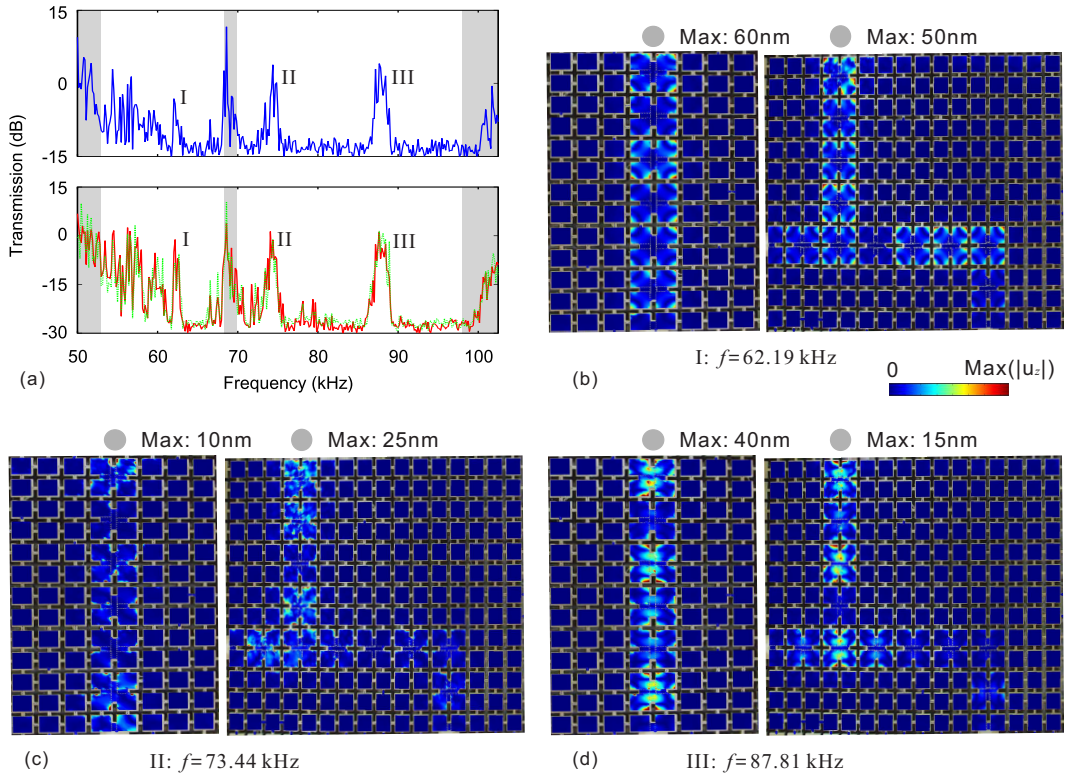
Figure 5: Experimental observation of Lamb wave propagation in the sample of Fig. 4. (a) The transmission through the waveguide (blue line: W1) and through the splitter (red line: S1, green line: S2) is shown as a function of frequency. Transmission is measured for the vertical component of displacement |u_z| and is normalized to its value at low frequency. The gray areas indicate the passing bands for perfect PC slab. Panels (b)-(d) show field distributions of displacement measured at chosen frequencies of the three passing frequency ranges labeled I-III in (a). In each panel, the left and right subplots are for the straight waveguide or the wave splitter, respectively. The wave source position is indicated by the gray disk. The color scale is for amplitude of z -displacement normalized with respect to the maximum amplitude (Max).
