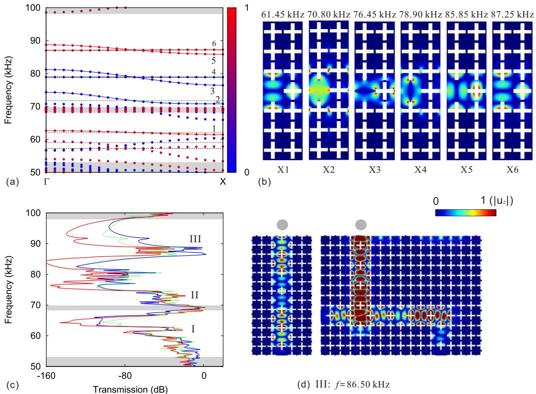
Figure 6: Finite element analysis of dispersion and transmission for coupled-resonator elastic waveguides of Fig. 5. (a) The band structure is obtained from a supercell model of the periodic waveguide. Points are for finite element results. Solid lines are obtained by fitting to a theoretical model (see text). The horizontal dashed lines mark the resonant frequencies for an isolated cavity in the PC slab. The color scale represents from the in-plane modes (blue) to out-of-plane modes (red). The gray areas indicate the passing bands for the perfect PC slab. (b) The displacement distributions at the X point of the 6 Bloch waves labeled in (a) are shown. (c) The numerical transmission through the straight waveguide and the wave splitter is plotted as a function of frequency. Panel (d) shows the displacement distributions at a chosen frequency inside passing range III. The color scale in panels (b) and (d) is for amplitude of z -displacement normalized with respect to the maximum amplitude (Max).
