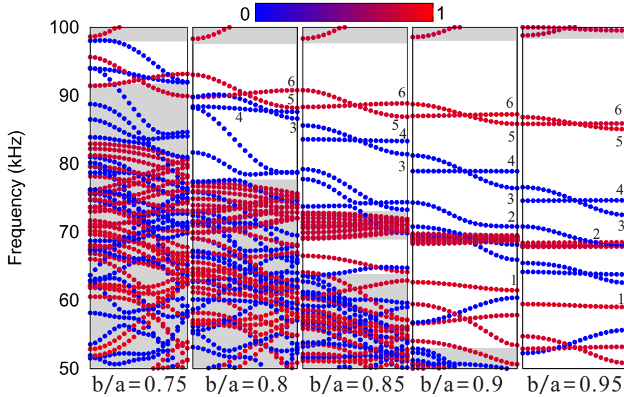
Figure 9: Band structures of CREWs with different relative hole lengths ( c/a = 0.2 , h/a = 0.4 ). The color scale measures the polarization and varies from in-plane modes (blue) to out-of-plane modes (red). The gray areas indicate the passing bands for the corresponding perfect PC slab.
