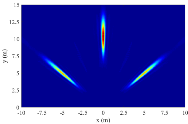
Fig. 4 Imaging result of three targets obtained by cross-correlation based BP algorithm.
