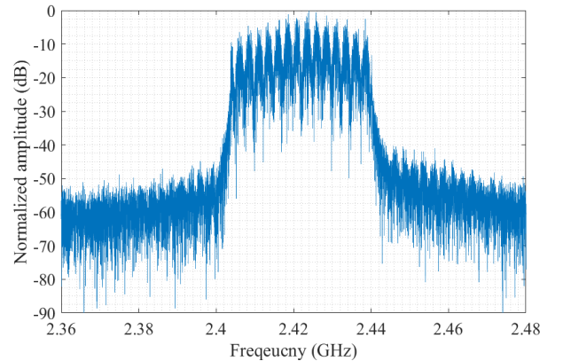
Fig. 2 Spectrum of real IEEE 802.11n signal with 40 MHz bandwidth used in the simulations.
