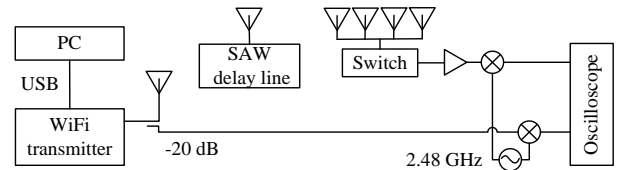
Fig. 9 Configuration of WiFi based passive sensor detection.
