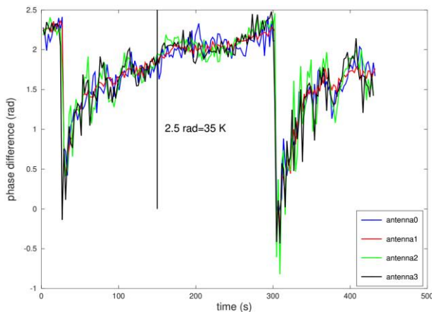
Fig. 12 Temperature variation observed on the 4 antennas facing a SAW delay line cooled twice by a freezing spray at dates 20 and 300 s.
