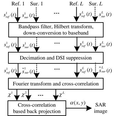
Fig. 1 Signal processing chain for WiFi based passive SAR imaging.
