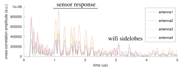
Fig. 11 WiFi based measurement of a passive sensor using IEEE 802.11n signal with 20 MHz bandwidth.
