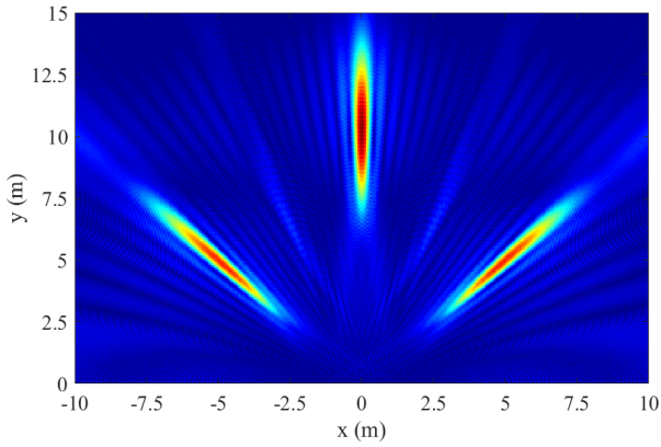
Fig. 3 Imaging result of three targets obtained by BP algorithm.
