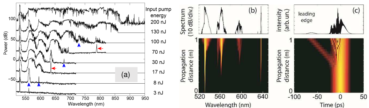
Figure 1 (a) Output experimental spectra with increasing input pump energy. Spectra are separated by 25 dB for better clarity. Resolution of OSA is 0.5 nm, except the highest energy with 2 nm. See text for explanation of blue and red arrows. (b) and (c) Numerical simulations of the generalized nonlinear Schrödinger equation including the Raman spectrum of Toluene and the dispersion in both the spectral and time domains.
