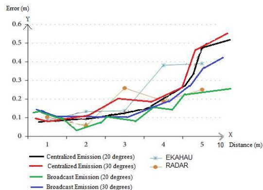
Figure 9 Accuracy of each scenario and comparison between our simulation and the RADAR and EKAHAU one
