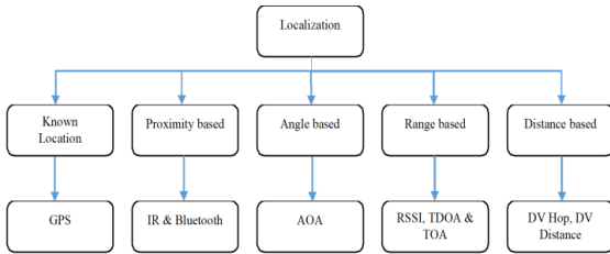
Figure 3 Localization- based Techniques
