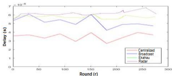
Figure 6 Delay comparison between the centralized and the broadcast emissions
