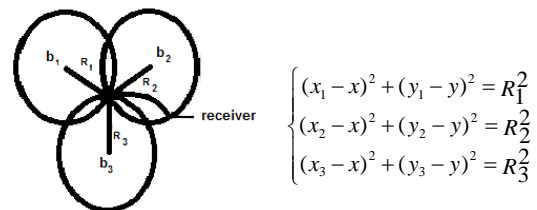
Figure 1 Trilateration-based Positioning
