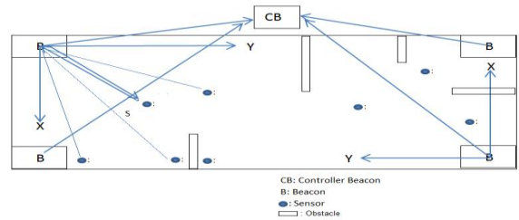
Figure 5 Broadcast Emission Scenario Table 3 Information on a CB about each Target Position According to each Related Beacon
