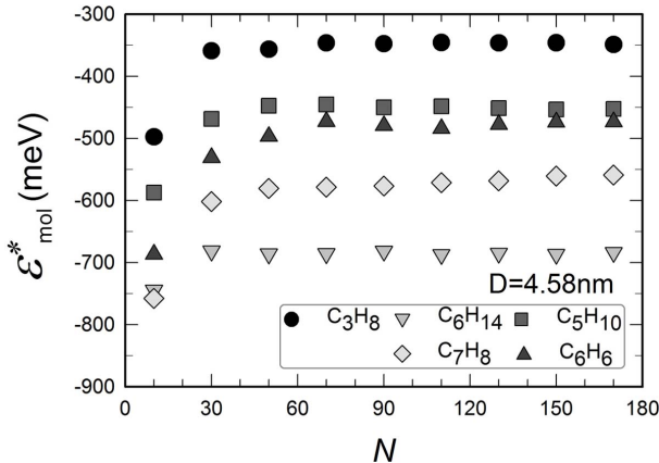
Figure 8. Adsorption energy per molecule versus the number N of organic molecules adsorbed on a nanoparticle of 4.58 nm in diameter.
