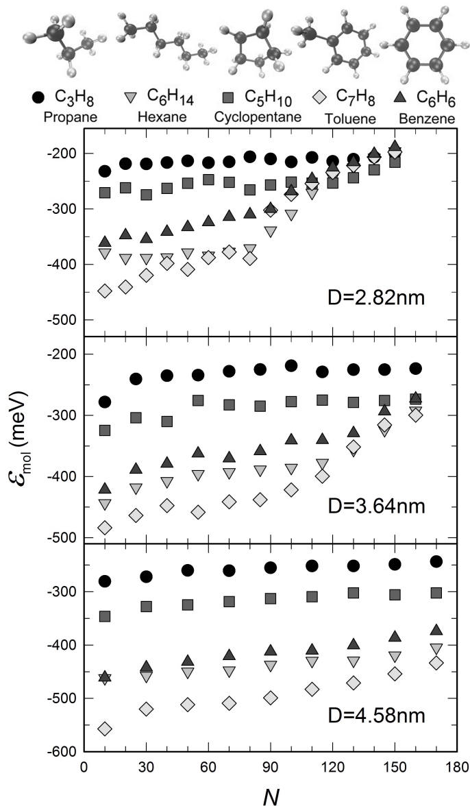
Figure 2. Adsorption energy per molecule versus the number N of five different organic molecules adsorbed on three nanoparticles of different sizes.
