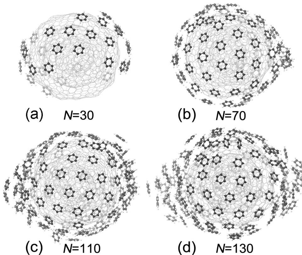
Figure 6. Atomistic configurations of the adsorbed benzene molecules on a carbon nanoparticle D = 2.82 nm with different surface coverages with (a) N = 30 , (b) N = 70 , (c) N = 110 , (d) N = 130 . The carbon and hydrogen atoms in benzenes are represented by black and white spheres, respectively.
