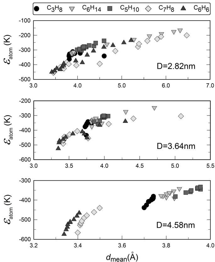
Figure 4. Adsorption energy per atom versus mean atomistic adsorbate-substrate spacing for various molecule numbers on three nanoparticles of different sizes.
