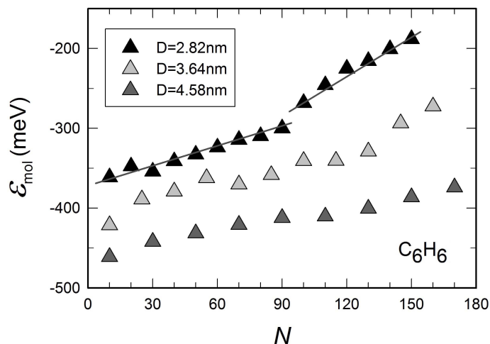
Figure 5. Adsorption energy per molecule as a function of the number N of C_6H_6 adsorbed on three nanoparticles of different sizes.
