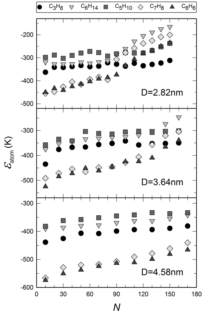
Figure 3. Adsorption energy per atom (in Kelvin) versus the number N of organic molecules for the five molecule types on three nanoparticles of different sizes.
