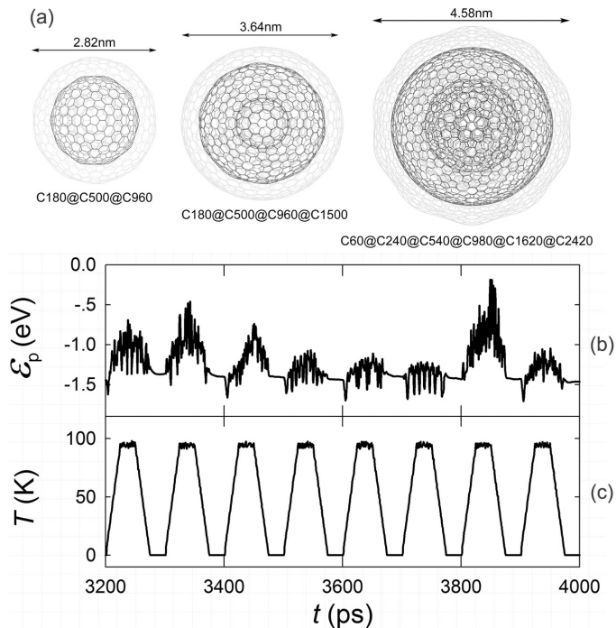
Figure 1. (a) Atomistic configurations of three “Russian doll” carbon nanoparticles studied in this work. (b-c) Variation of the potential energy \epsilon_p and temperature T of a sample during a simulation for instance. The zero-potential value of \epsilon_p is set to be -21767.0 eV.
