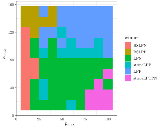
Figure 4: Best average NM , \Phi_{\max} = 350 .
