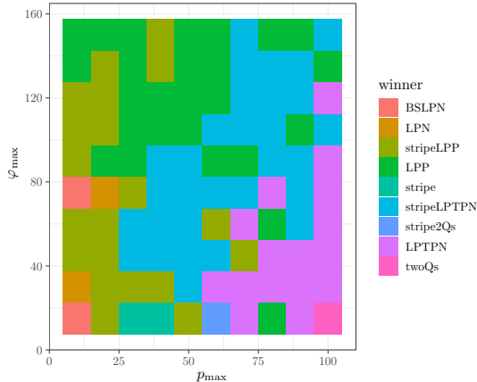
Figure 5: Best average NM , \Phi_{\max} = 700 .
