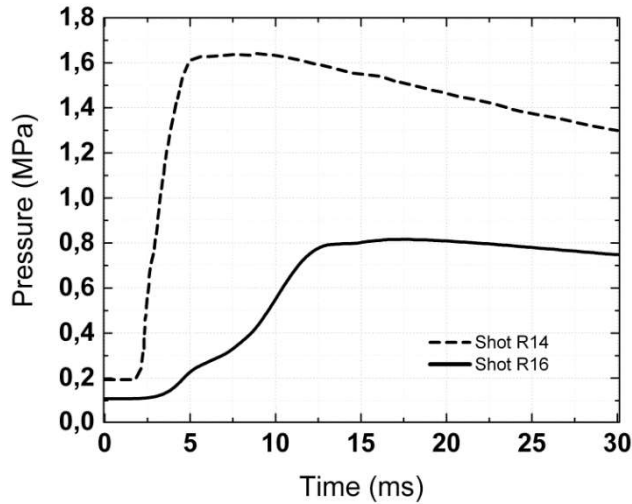
FIG.9: Typical measured pressures for Shots R16 ( P=7.9 bar) and R14 ( P=16.1 bar)
