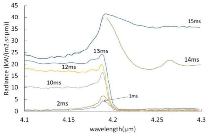
FIG.13: Measured pressure (13a) and radiances in experiment L1 in the IR range at several times (13b)
