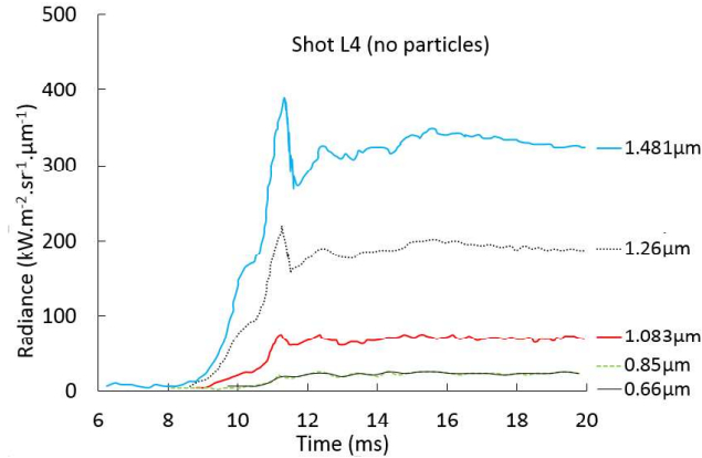
FIG. 15: Results for shots L4 and L8
