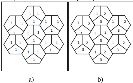
Figure 1. Seven-cell hexagonal layout. a) 1 \times 3 \times 1 b) 1 \times 3 \times 3
