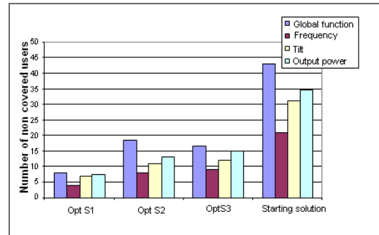
Figure 11. Comparison between frequency, tilt and output power optimization: Sites processed according their storage in data file; stopping criteria when there is no improvement
