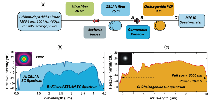
Fig. 3. a) Experimental setup for mid-infrared SC generation in a cascaded silica-ZBLAN-chalcogenide optical fiber system. b) Experimental SC spectra at the ZBLAN fiber output (light blue) and after the long-pass Germanium filter (dark blue). c) Experimental SC spectrum at the chalcogenide fiber output (yellow). The insets show the optical mode profiles out of both the ZBLAN (b) and chalcogenide (c) optical fibers. Taken from Ref. [78].
