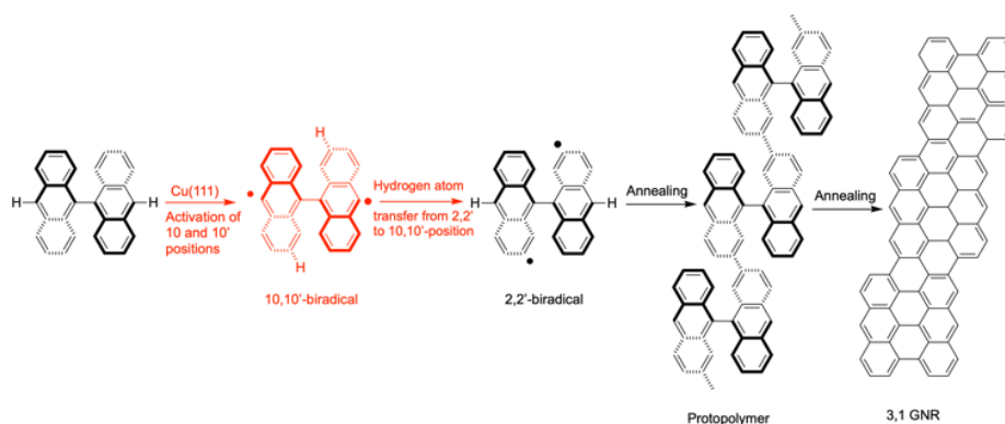
Figure: Completed reaction mechanism for the growth of (3,1) GNR induced by a two-step annealing of BA molecules on a Cu(111) surface. The formation of 10,10'-biradical (in red), followed by radical transposition, is added as initial step.
