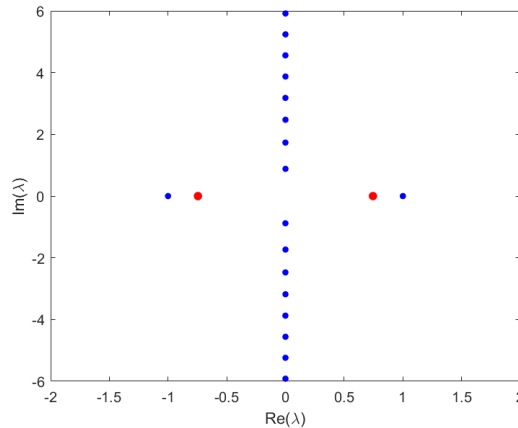
FIGURE 2. The union \Sigma_{AB}^{(P)} \cup \Sigma_{AB}^{(A)} of the Lax spectra in L_{\text{per}}^2(0, L) and L_{\text{antiper}}^2(0, L) for AB. The red dots represent the eigenvalues \{+\lambda_0, -\lambda_0\} .
