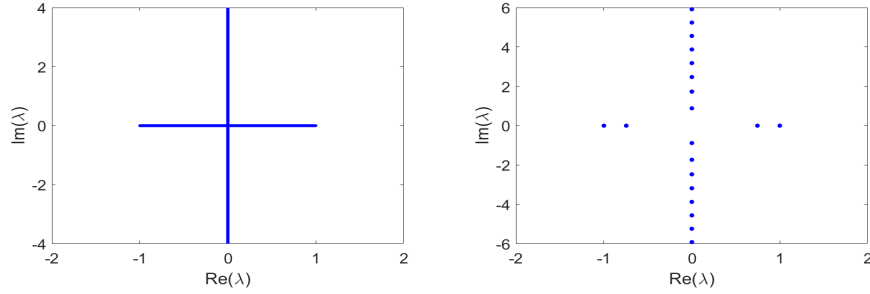
FIGURE 1. Left: The Lax spectrum \Sigma_0 in L^2(\mathbb{R}) . Right: The union \Sigma_0^{(P)} \cup \Sigma_0^{(A)} of the Lax spectra in L^2_{\text{per}}(0, L) and L^2_{\text{antiper}}(0, L) for some positive L \notin \pi\mathbb{N} .
