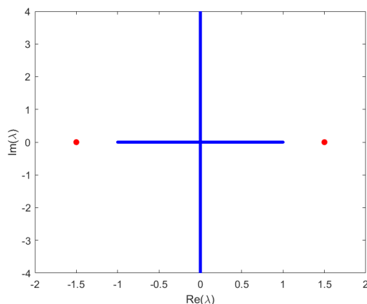
FIGURE 3. The Lax spectrum \Sigma_{\text{KMB}} in L^2(\mathbb{R}) for KMB.
