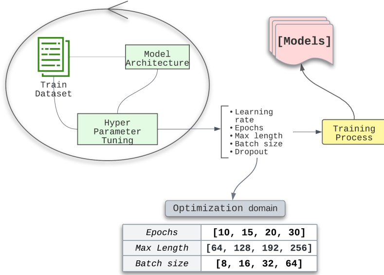
Figure 4: FineTuning Process.
