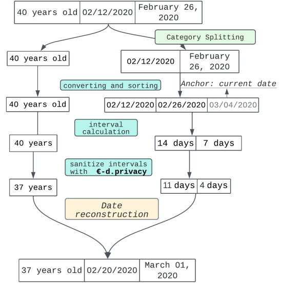
Figure 5: Example of date substitution process on the thread example.
