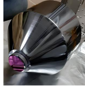
Figure 1: The horizontal cavity spacer has a biconic shape with specific cut angles to reduce the sensitivity to accelerometric noise.
