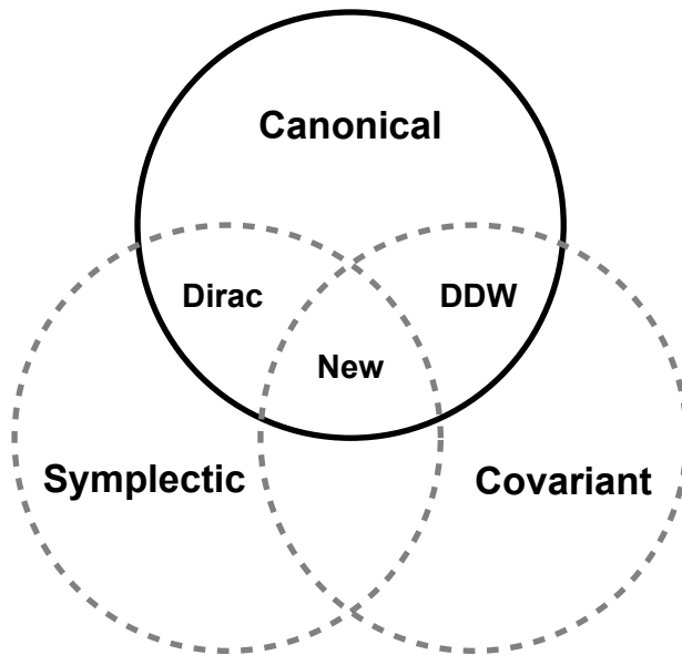
FIG. 1. A comparison of the Dirac \mathcal{H}_D , De Donder-Weyl \mathcal{H} , and the new covariant \mathcal{H}_{new} Hamiltonian densities, focusing on whether these formulations are covariant or symplectic. All Hamiltonian formulations contain a canonical momentum, but not all are covariant or symplectic. These three Hamiltonian formulations arise from the same Lagrangian density \mathcal{L} .
