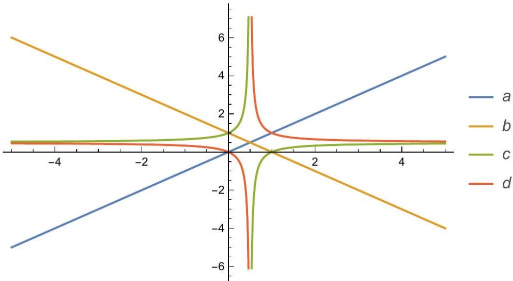
FIG. 2. The solution for coefficients a, b, c, and d are shown as a function of a such that both the classical and quantum phase space coordinates equal to Planck's constant times their corresponding wavenumbers.
