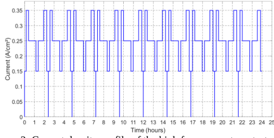
Figure 2: Current density profile of the high frequency stress test protocol
