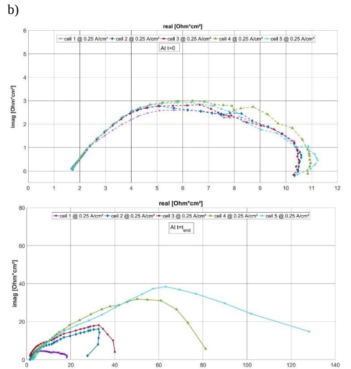
Figure 6: a) Long-term test results for the high frequency stress test b) EIS results
