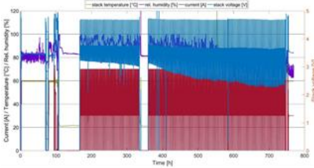
Figure 7: Long-term test results for the high frequency and amplitude stress test with conditioning phase (t=0 until t=180h)
