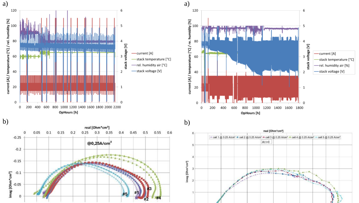
Figure 5: a) Long-term test results for the reference profile b) EIS results
