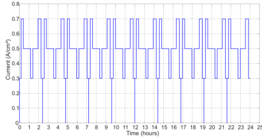
Figure 3: Current density profile of the high frequency and magnitude stress test protocol
