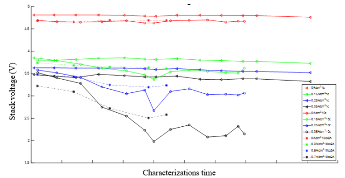
Figure 8: Stack voltage evolution trend with time
