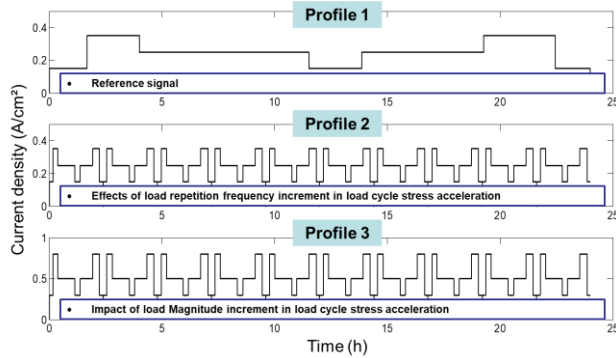
Figure 4: Three profiles tested on short-stacks
