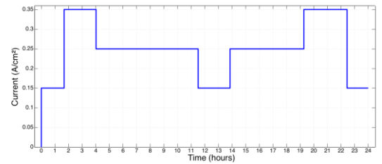
Figure 1: Current density profile of the reference test protocol
