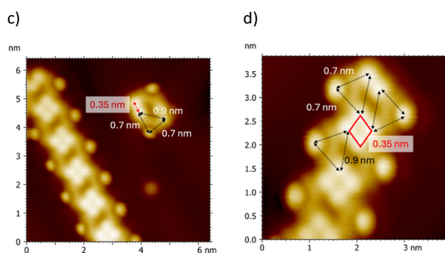
Figure 1. Different nanostructures observed after the deposition of 0.3 monolayer of DIDEc molecule onto an Au(111) surface at 80 K. (a) CPK model of the 3,6-diiodo-9-ethylcarbazole (DIDEc) molecule. (b) STM image ( 6.5 \times 6.5 \text{ nm}^2 , V_s = 0.3 \text{ V} , I_t = 12 \text{ pA} , 9K) showing a bean-shaped protrusion surrounded by three bright spots arranged in an isosceles triangular geometry, with two sides measuring 0.7 nm and one side 0.9 nm. (c) STM image ( 6.4 \times 6.4 \text{ nm}^2 , V_s = 0.2 \text{ V} , I_t = 180 \text{ pA} , 9K) showing two bean-shaped protrusions arranged face-to-face along the longest side, separated by 0.35 nm. The four closely spaced protrusions appear brighter than the two more distant ones. (d) STM image ( 3.9 \times 3.9 \text{ nm}^2 , V_s = -1.0 \text{ V} , I_t = 31 \text{ pA} , 9K) showing a row composed of the features observed in (c). The four brightest protrusions are arranged in a diamond-shaped configuration, with sides measuring 0.35 nm.
