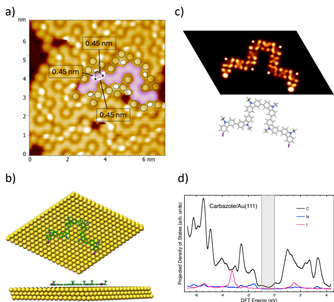
Figure 3. (a) STM image ( 6.5 \times 6.5 nm 2 , V_s = 0.1 V, I_t = 40 pA, 9K) showing nanostructures formed after deposition of 0.3 monolayers of DIDEDEC on Au(111) at 80 K, followed by thermal annealing at 378 K for 30 min. A compact network of continuous backbone (highlighted in pink), surrounded by bright protrusions (black ellipses) and larger ones (dashed black circles), is visible. Bean-shaped features (highlighted in white) appear within the backbone, forming equilateral
