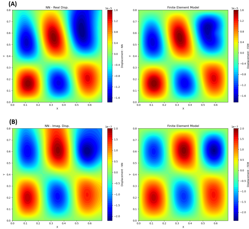
Figure 4: Real (A) and imaginary (B) components of displacements at 130 Hz over the measured region for the homogeneous plate: PINN estimates (left) and FEM reference (right)
