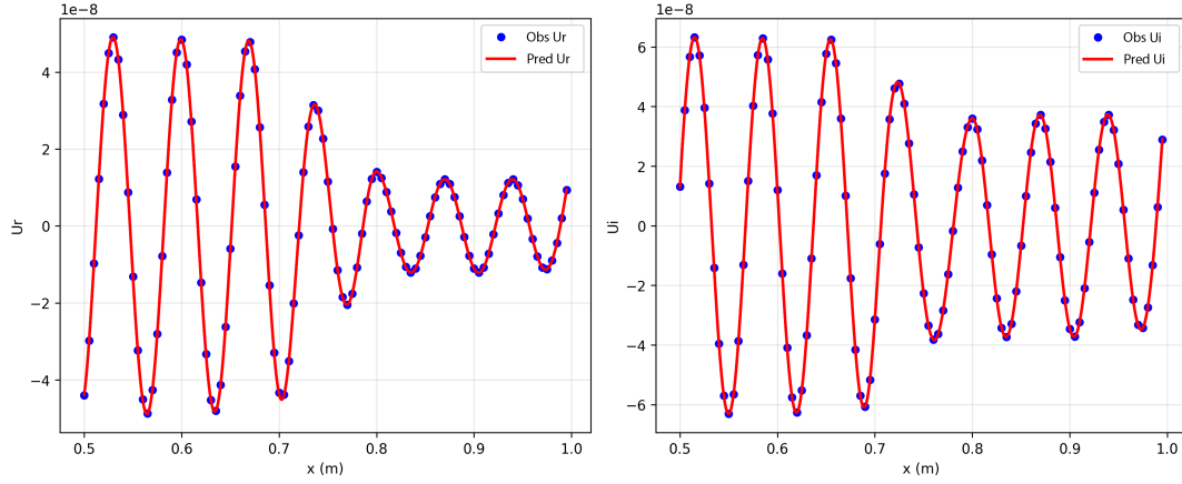
Figure 2: Observed vs. predicted complex displacements at 4 kHz over the measured region for the 6 plateaus model
