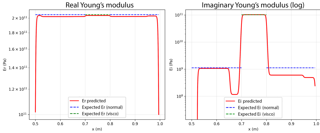
Figure 3: Results with 6 learnable bounded plateaus: predicted real (left) and imaginary (right) parts of the modulus. Clean plateaus and physically plausible transitions are obtained.
