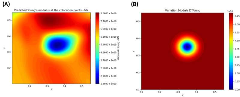
Figure 7: Identified elastic modulus of the non-homogeneous plate (A) and reference (B)
