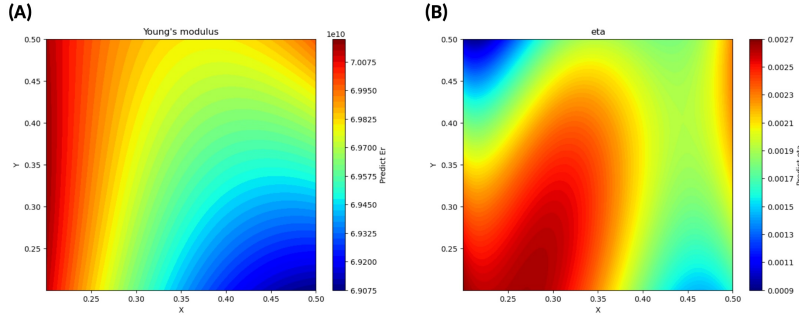
Figure 5: Identified properties of the homogeneous plate: elastic modulus (A) and loss factor (B)
