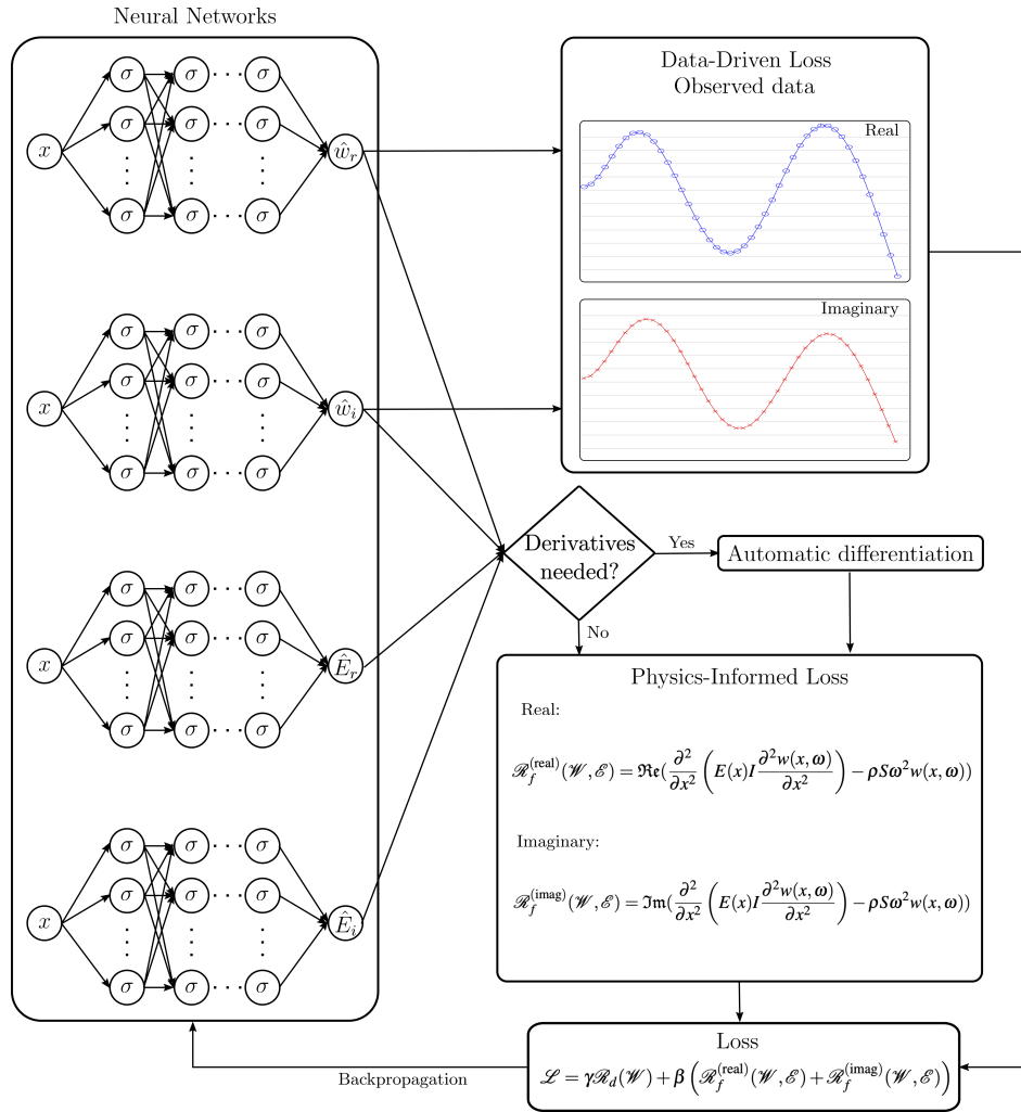
Figure 1: PINN framework
