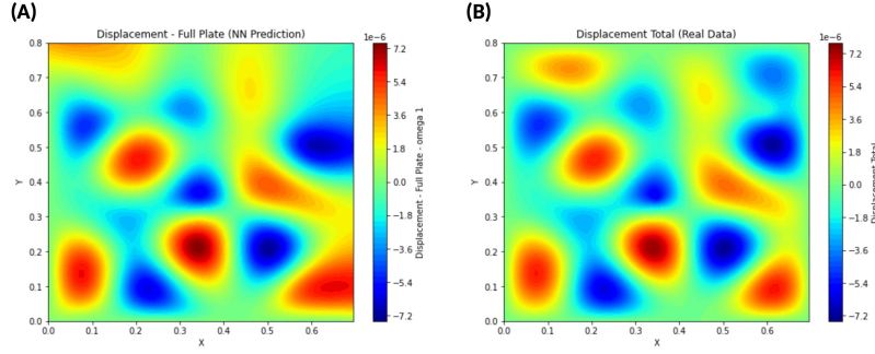
Figure 6: Displacement at 295 Hz over the measured region for the non-homogeneous plate: PINN estimates (A) and FEM reference (B)
