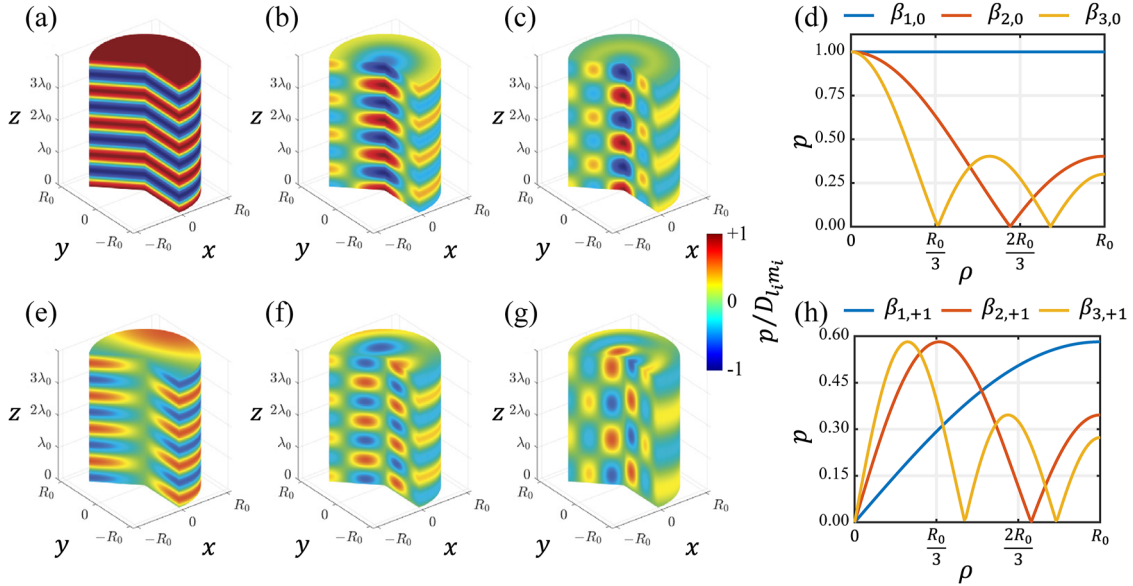
FIG. 2. Theoretical spatial distribution of normalized sound pressure for traveling CBMs with azimuthal index m = 0 and [(a)–(d)] m = +1 [(e)–(h)]. (a)–(c) CBMs with m = 0 and radial wavenumbers \beta_{1,0} = 0 \text{ m}^{-1} , \beta_{2,0} = 25.5 \text{ m}^{-1} , and \beta_{3,0} = 46.8 \text{ m}^{-1} , respectively. (d) Amplitude distributions along the radius \rho for CBMs with m = 0 and \beta_{1,0} = 0 \text{ m}^{-1} (blue curve), \beta_{2,0} = 25.5 \text{ m}^{-1} (red curve), and \beta_{3,0} = 46.8 \text{ m}^{-1} (orange curve). (e)–(g) CBMs with m = +1 and radial wavenumbers \beta_{1,+1} = 12.3 \text{ m}^{-1} , (f) \beta_{2,+1} = 35.5 \text{ m}^{-1} , and (g) \beta_{3,+1} = 56.9 \text{ m}^{-1} , respectively. (h) Amplitude distribution along the radius \rho for CBMs with m = +1 and \beta_{1,+1} = 12.3 \text{ m}^{-1} (blue curve), \beta_{2,+1} = 35.5 \text{ m}^{-1} (red curve), and \beta_{3,+1} = 56.9 \text{ m}^{-1} (orange curve).
