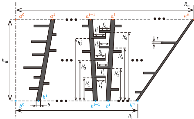
FIG. 5. Schematic of designed generalized acoustic impedance metasurface.
