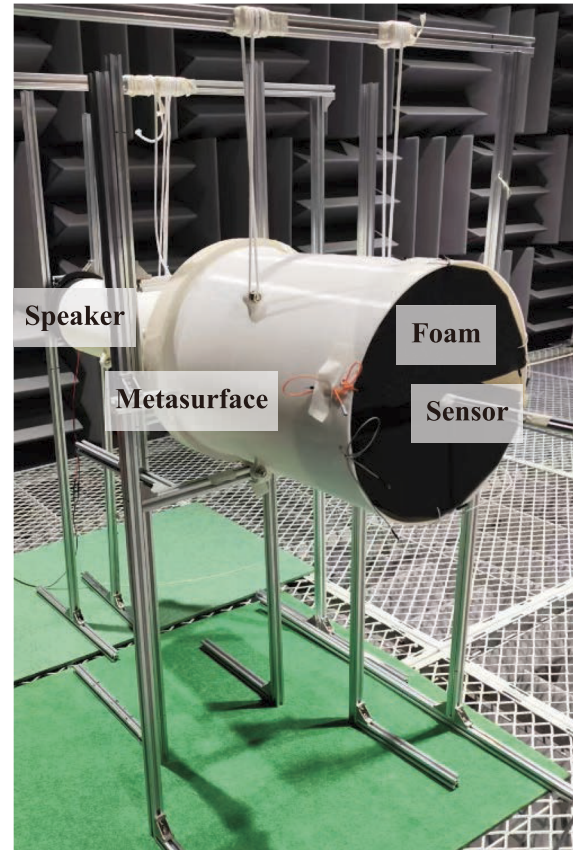
FIG. 7. Experimental setup for generation with a single speaker.
