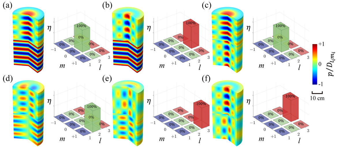
FIG. 3. Verification by numerical simulation of the operation of metasurfaces for CBM conversion. Normalized total pressure fields and orthogonal decompositions of the output signal are shown for conversion (a) from \beta_{1,0} to \beta_{2,0} , (b) from \beta_{1,0} to \beta_{3,0} , (c) from \beta_{2,0} to \beta_{3,0} , (d) from \beta_{1,+1} to \beta_{2,+1} , (e) from \beta_{2,+1} to \beta_{3,+1} , and (f) from \beta_{3,+1} to \beta_{3,0} .
