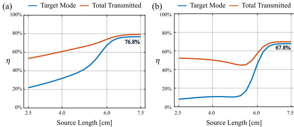
FIG. 9. Simulation results for the influence of different lengths of sound source on the efficiency of metasurfaces for (a) \beta_{1,0} \rightarrow \beta_{2,0} and (b) \beta_{1,0} \rightarrow \beta_{3,0} .
