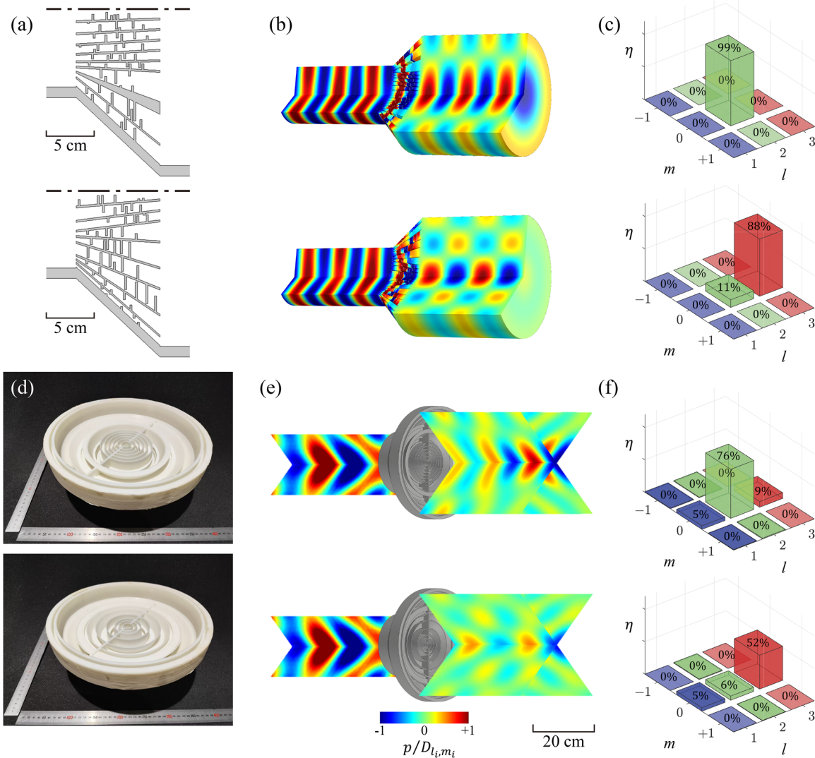
FIG. 4. Verification by numerical simulation and experiment of metasurfaces designed for CBM generation from a plane wave to CBMs with \beta_{2,0} and \beta_{3,0} . The metasurface designed by optimization (a) produces the simulated pressure field in (b), whose orthogonal decomposition is shown in (c). The fabricated metasurface (d) produces the experimental pressure field in (e), whose orthogonal decomposition is shown in (f).
