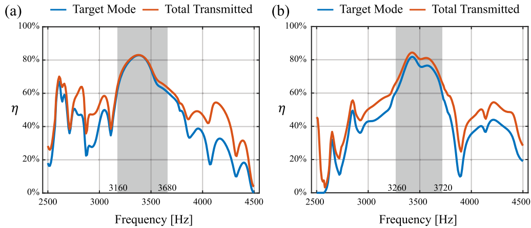
FIG. 8. Frequency-domain response of metasurfaces for (a) \beta_{1,0} \rightarrow \beta_{2,0} and (b) \beta_{1,0} \rightarrow \beta_{3,0} .
