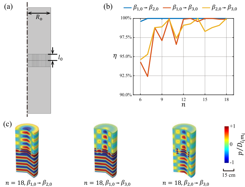
FIG. 6. Simulation results for the influence of different unit discretizations on metasurface efficiency. (a) Three-layer numerical model for simulation. (b) Influence of different numbers of discrete units on the efficiency of metasurfaces for \beta_{1,0} \rightarrow \beta_{2,0} (blue line), \beta_{1,0} \rightarrow \beta_{3,0} (orange line), and \beta_{2,0} \rightarrow \beta_{3,0} (yellow line). (c) Simulation results for metasurfaces with n = 18 .
