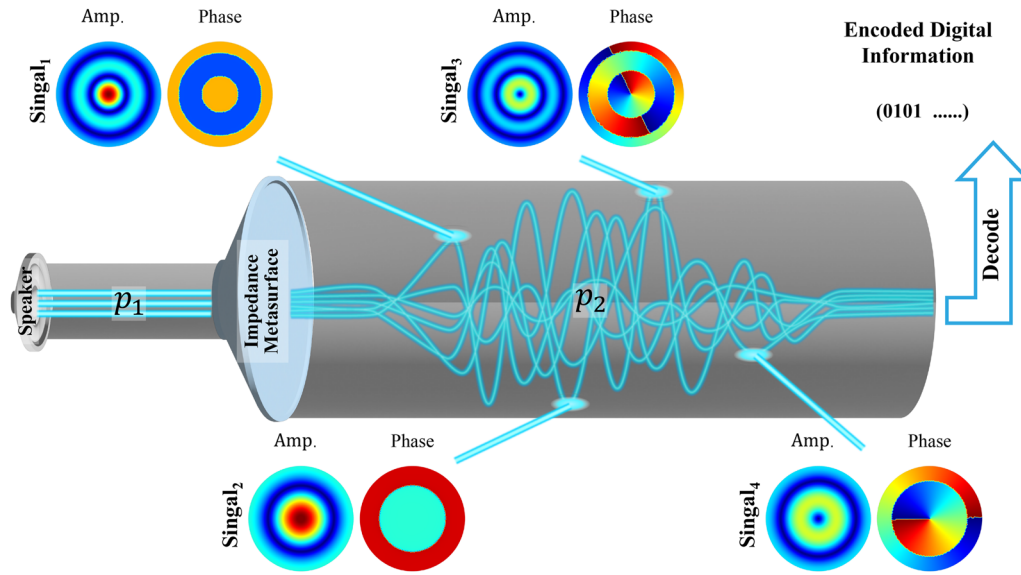
FIG. 1. Illustration of a generalized impedance metasurface for CBM generation. A metasurface with two unequal cross-sectional areas connects a fundamental planar wave field p_1 generated by a speaker and a field p_2 encoded with specific digital information through amplitude and phase modulation.
