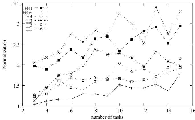
Figure 11: m = 5, p = 2 . Normalization with the MIP.
