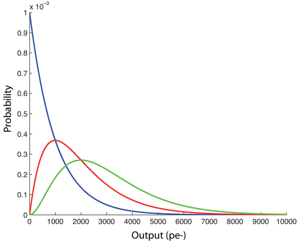
Figure 1: EMCCD output probabilities for a given number of input photons n = 1 (blue curve), n = 2 (red curve), and n = 3 (green curve), and for a mean gain of 1000.
