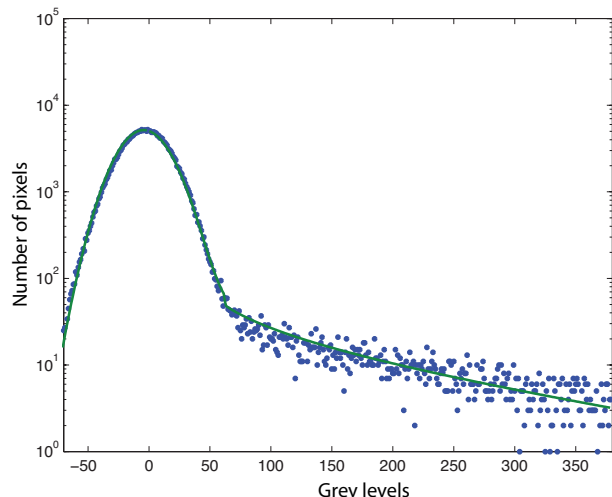
Figure 5: Histogram of grey levels for a dark image of the Hamamatsu EMCCD (blue dots) and corresponding fit (green curve).
