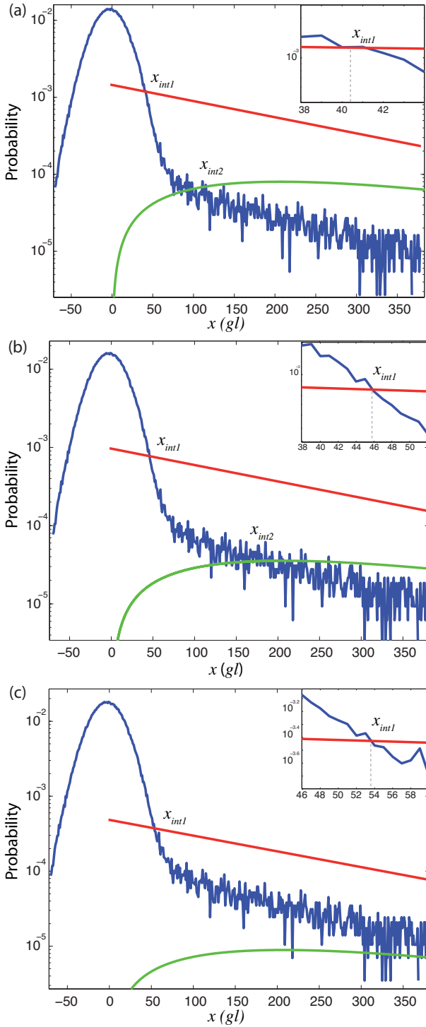
Figure 6: Probabilities ( p(x|0)(1 - \mu) in blue, p(x|1)\mu in red, and p(x|2)\mu^2/2 in green) involved in the thresholding procedure for the Hamamatsu EMCCD demo, for three different cases of illumination; (a) \mu = 0.3ph/pix , (b) \mu = 0.2ph/pix , (c) \mu = 0.1ph/pix .
