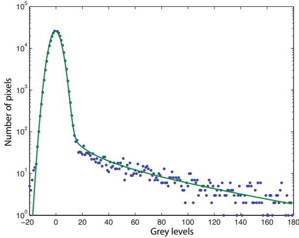
Figure 2: Histogram of grey levels for a dark image of the Andor EMCCD (blue dots) and corresponding fit (green curve).
