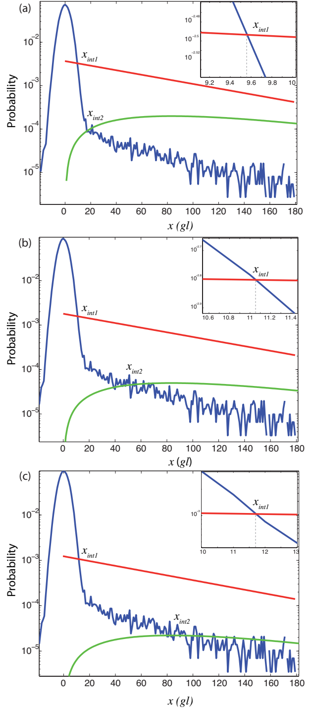
Figure 3: Probabilities ( p(x|0)(1 - \mu) in blue, p(x|1)\mu in red, and p(x|2)\mu^2/2 in green) involved in the thresholding procedure for the Andor EMCCD, for three different cases of illumination; (a) \mu = 0.3 \text{ ph/pix} , (b) \mu = 0.15 \text{ ph/pix} , (c) \mu = 0.1 \text{ ph/pix} . In the inset, zoom of the region of intersection between p(x|0)(1 - \mu) and p(x|1)\mu .
