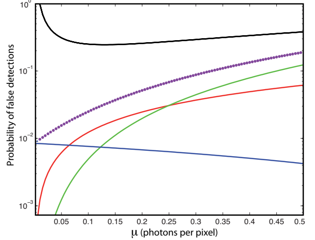
Figure 4: False detection probabilities P_0 (blue curve), P_1 (red curve) and P_2 (green curve), and total probability of error (dotted curve), plotted as a function of \mu , for T = 11gl in the case of the Andor EMCCD. The black solid curve represents the relative total error in detection (i.e. total probability of error divided by \mu ).
