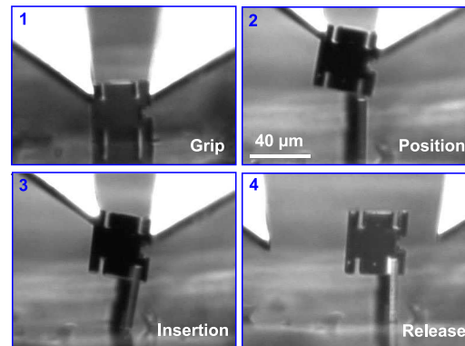
Fig. 33 Insertion assembly.
