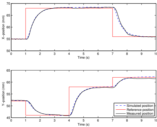
Fig. 15 Experimental results.
