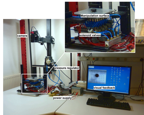
Fig. 13 Overview of the experimental setup.
