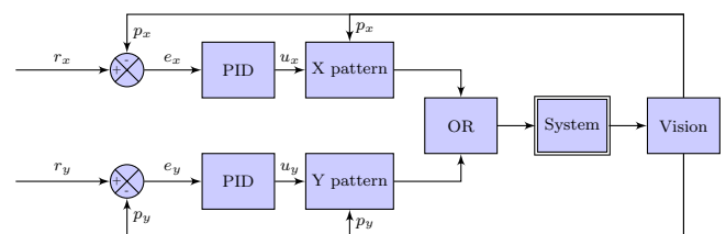
Fig. 14 Control architecture.
