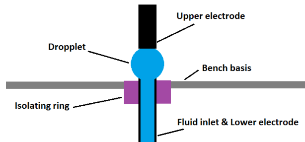
Figure 7. Resistive measurements, measuring electrodes, Keyence laser distance. Sensor & laser line, injection syringe and position of the droplet.
