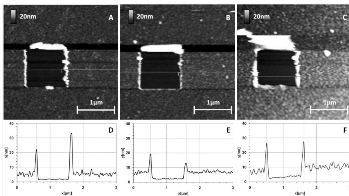
Figure 6. AFM images after strong scraping applied to GaAs biofunctionalized surfaces. Images and corresponding sections: 0% MHDA (A,D); 100% MHDA (B,E); and 10% MHDA (C,F).
