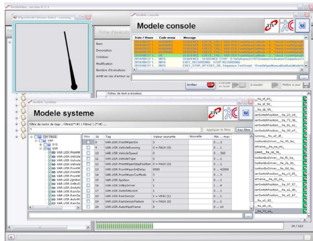
Fig. 6 Clemessy TestInView interface
