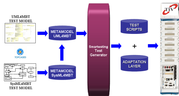
Fig. 3 VETESS final toolchain.
