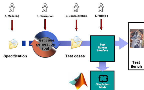
Fig. 1 Model-Based Testing process.
