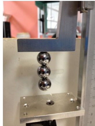
Figure 5: The 3 magnets in position vertical.
