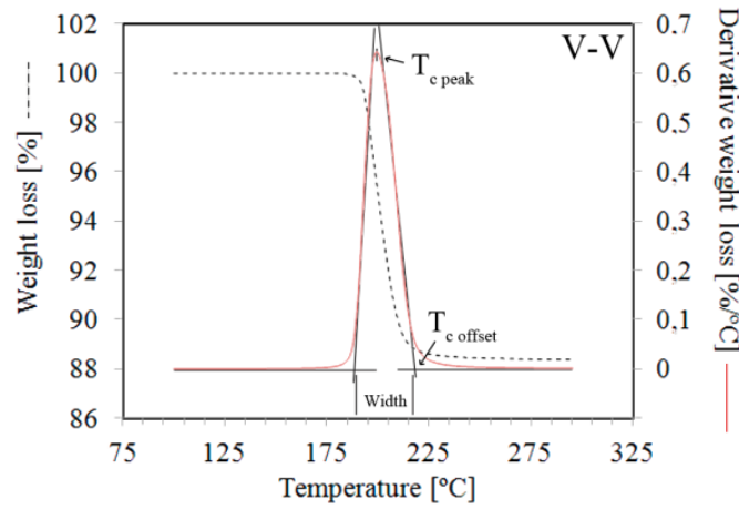
Figure 7 TGA weight loss (dashed line) associated with the Invar 36 ferromagnetic to paramagnetic transition. The derivative of the curve represents the characteristic Curie's temperature peak defined by its maximum, the offset and the width.
