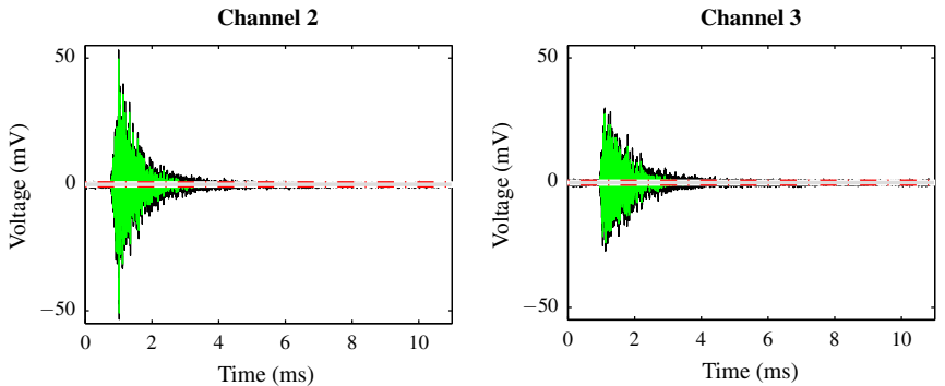
Figure 4 : Comparison of the raw and denoised signals of channels 2 and 3 after a PLB under a low noise level. (—) Raw signals; (—) denoised signals; and (---) threshold level.
