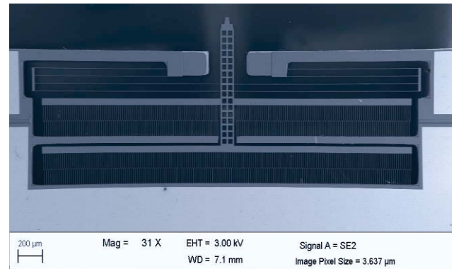
Figure 8. Alternative design for micro-actuator with two set of electrostatic comb-drives.
