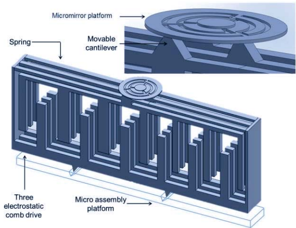
Figure 2. Schematic of micro-manipulator design for robot-assisted laser phonomicrosurgery with electrostatic micro-actuators [17].
