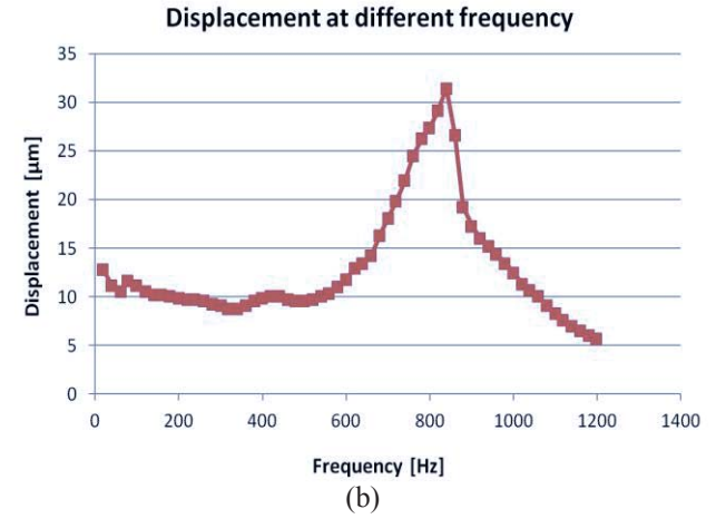
Figure 12. Dynamics analysis for electrostatic actuators at different frequencies (a) a device with single-beam suspensions (b) a device with double-folded-beam suspensions.
