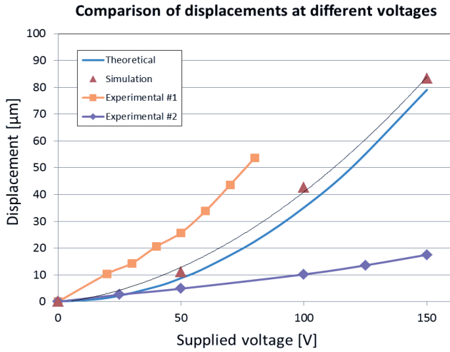
Figure 10. Comparison of performances between theoretical results, simulation results, and experimental results. Experimental result #1 (orange dots) is a device with double-folded-beam suspensions and experimental result #2 (purple dots) is a device with single-beam suspensions.
