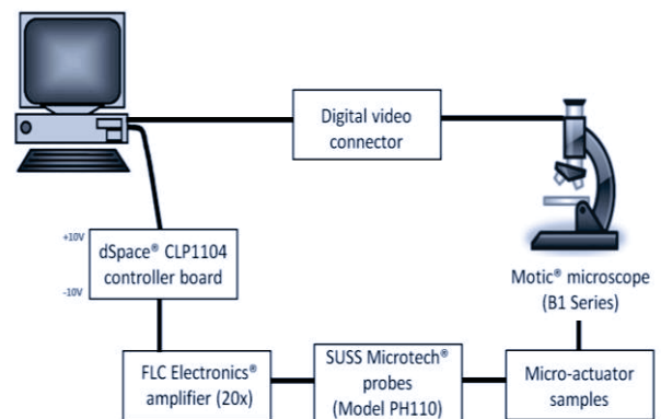
Figure 9. Schematic of the apparatus used for measuring static displacement of electrostatic micro-actuators.
