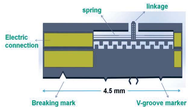
Figure 3. Micro-manipulator with electrostatic actuators with markers and breaking parts.
