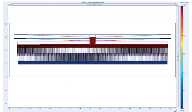
Figure 5. COMSOL ® simulation result for single-beam suspensions (Design A) showing a displacement of 12 \mu\text{m} at 50 V.
