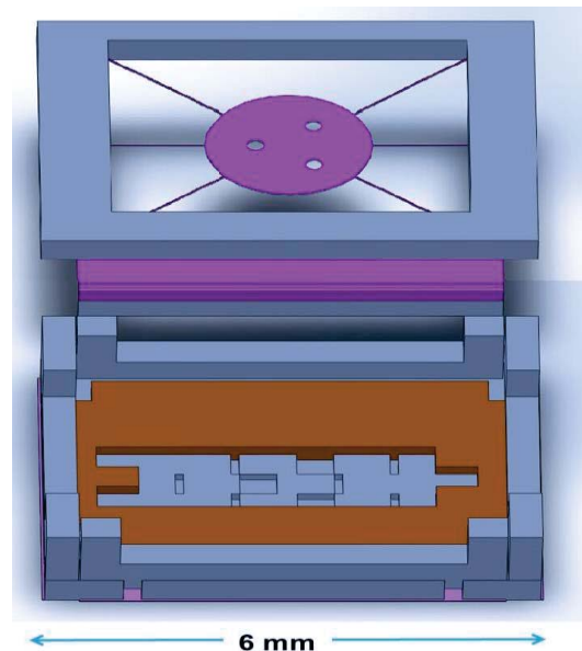
Figure 4. Micro-assembly block with markets and slots used for placing three electrostatic actuators..
