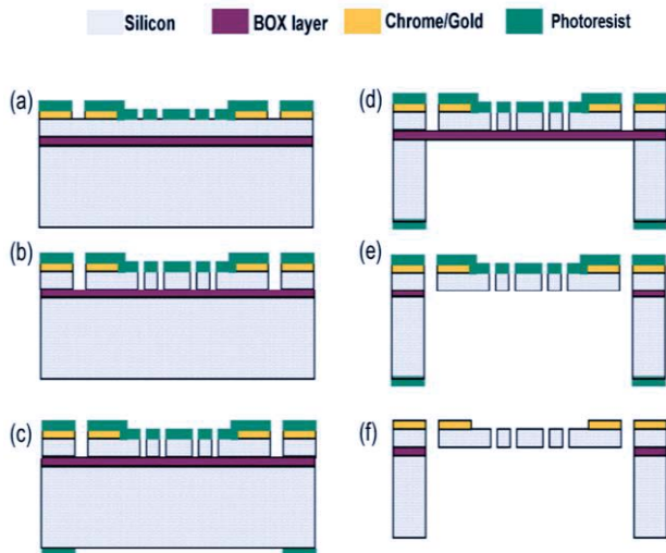
Figure 6. Microfabrication process of electrostatic actuators and mirror for phonomicrosurgery.
