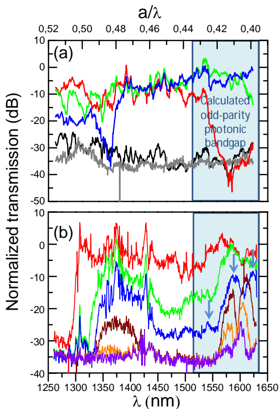
Figure 3. Measured normalized spectra for TM-polarized light and for different values of d and PCS waveguide lengths. (a) d=A (black), d=1.2A (red), d=1.4A (green), d=1.6A (blue). The grey curve corresponds to a perfect crystal but with incidence along the \Gamma X direction. The total length of the PCS region (with or without waveguide) is 10\ \mu\text{m} ; (b) Waveguides with d=1.6A and total length of 10\ \mu\text{m} (red), 30\ \mu\text{m} (green), 50\ \mu\text{m} (blue), 100\ \mu\text{m} (brown), 150\ \mu\text{m} (orange), and 200\ \mu\text{m} (violet). The arrows highlight the observed transmission peaks in the 50\ \mu\text{m} waveguide response.
