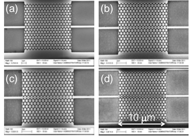
Figure 2. Scanning electron microscopy images of the fabricated waveguides along \Gamma J : (a) d=A (no waveguide), (b) d=1.2A (c) d=1.4A (d) d=1.6A .
